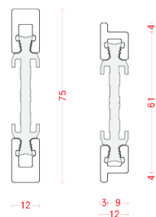
BT 7512PU-08
