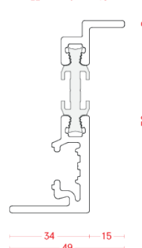
BT 8212ZR-08
