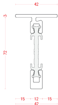
BT 7512T-08
