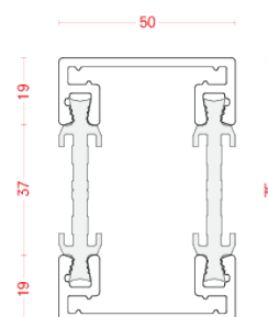
BT 7550T-08
