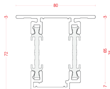
BT 7550T-08
