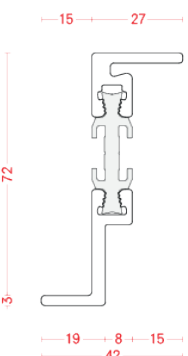
BT 7512ZR-08
