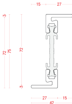
BT 7512Z-08
