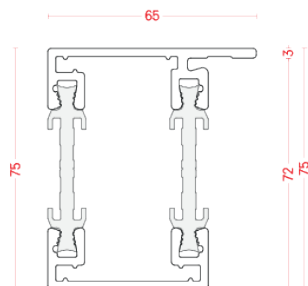
BT 7550LF-08
