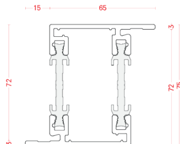
BT 7550ZF-08
